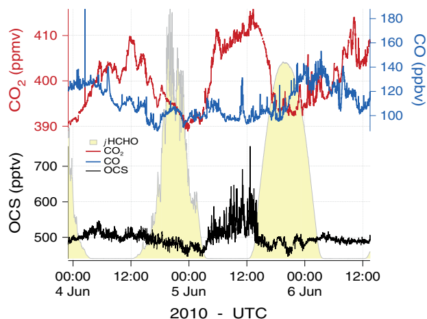
Figure 3. Time Series of CO 2 (red), CO (blue), OCS (black) and the photolysis rate of formaldehyde ( j HCHO, used as a proxy for daylight) (yellow) around Sacramento. The influence of photosynthetic uptake of OCS and CO 2 was seen as parallel decline in OCS and CO 2 on 4 June (up to 02:00 UTC on 5 June). Then both increased due to strong local emissions of OCS and CO 2 from a nearby wetland, overnight on 5 June. On this night, wind speeds varied between 1 and 4 m s -1 . No OCS increase was associated with increasing CO when sampling downwind of a petrochemical refinery (6 June).
